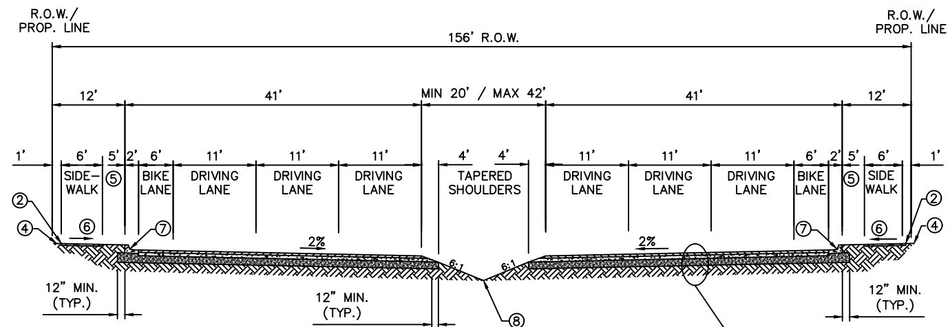
TYPICAL STREET SECTION - 6 LANE PRINCIPAL ARTERIAL INVERTED CROWN
