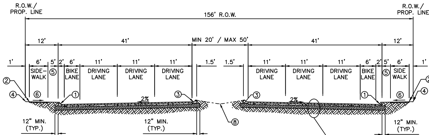
TYPICAL STREET SECTION - 6 LANE PRINCIPAL ARTERIAL
